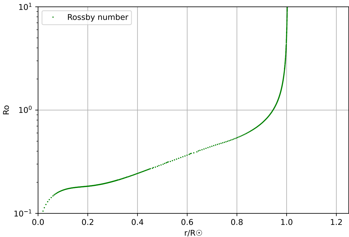
Rossby number, profile 148, age 4.91 \times 10^9
